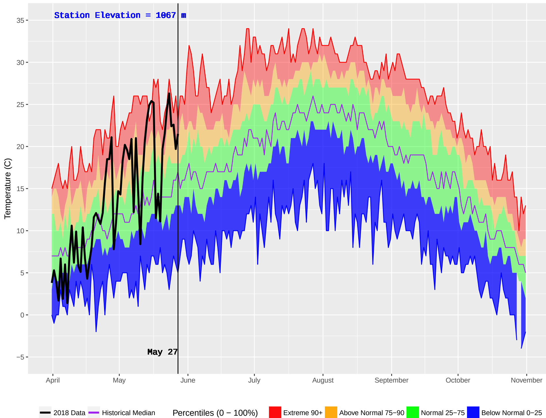
MCCUDDY (334) : Historical (1984–2016) and Current (2018) Noon Temperature
